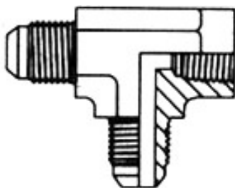
FEMALE RUN TEE
