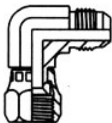
FEMALE ELBOW 90°
