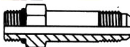
STRAIGHT THREAD EXTENDED CONNECTOR
