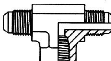
FEMALE BRANCH TEE
